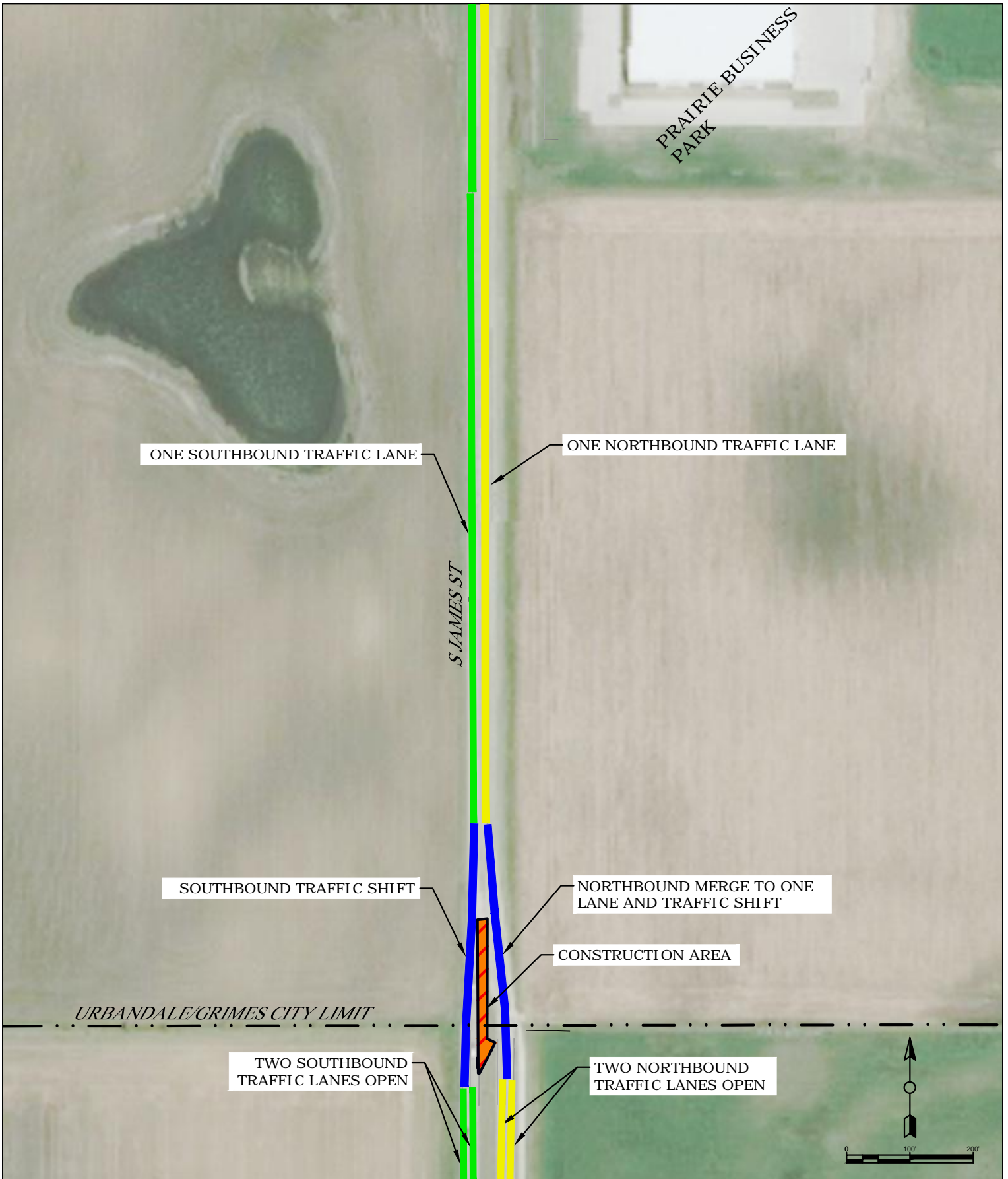
S JAMES & SE 37TH ST IMPROVEMENTS PROJECT PHASE 1 TRAFFIC CONTROL
