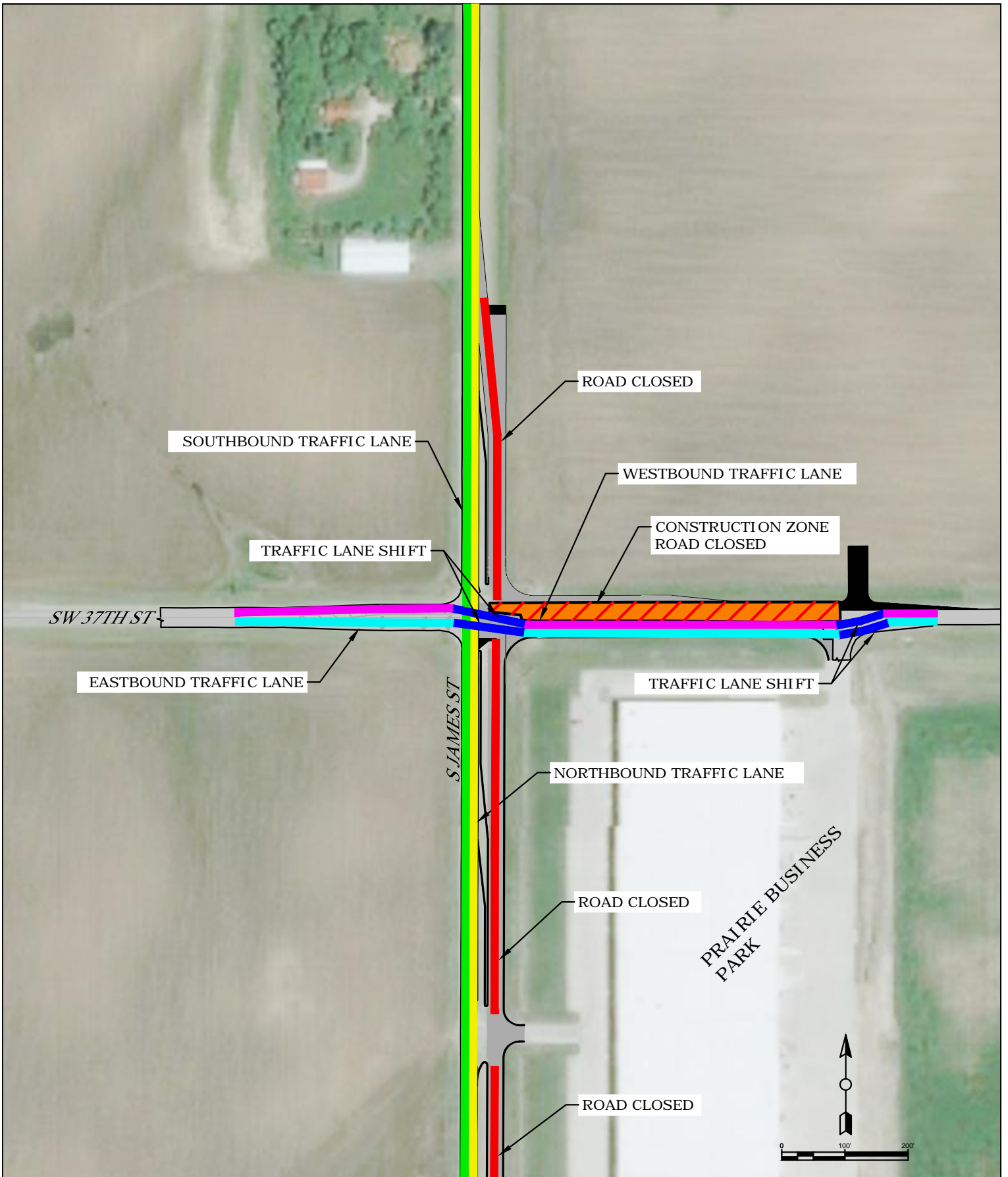
S JAMES & SE 37TH ST IMPROVEMENTS PROJECT PHASE 4 TRAFFIC CONTROL
