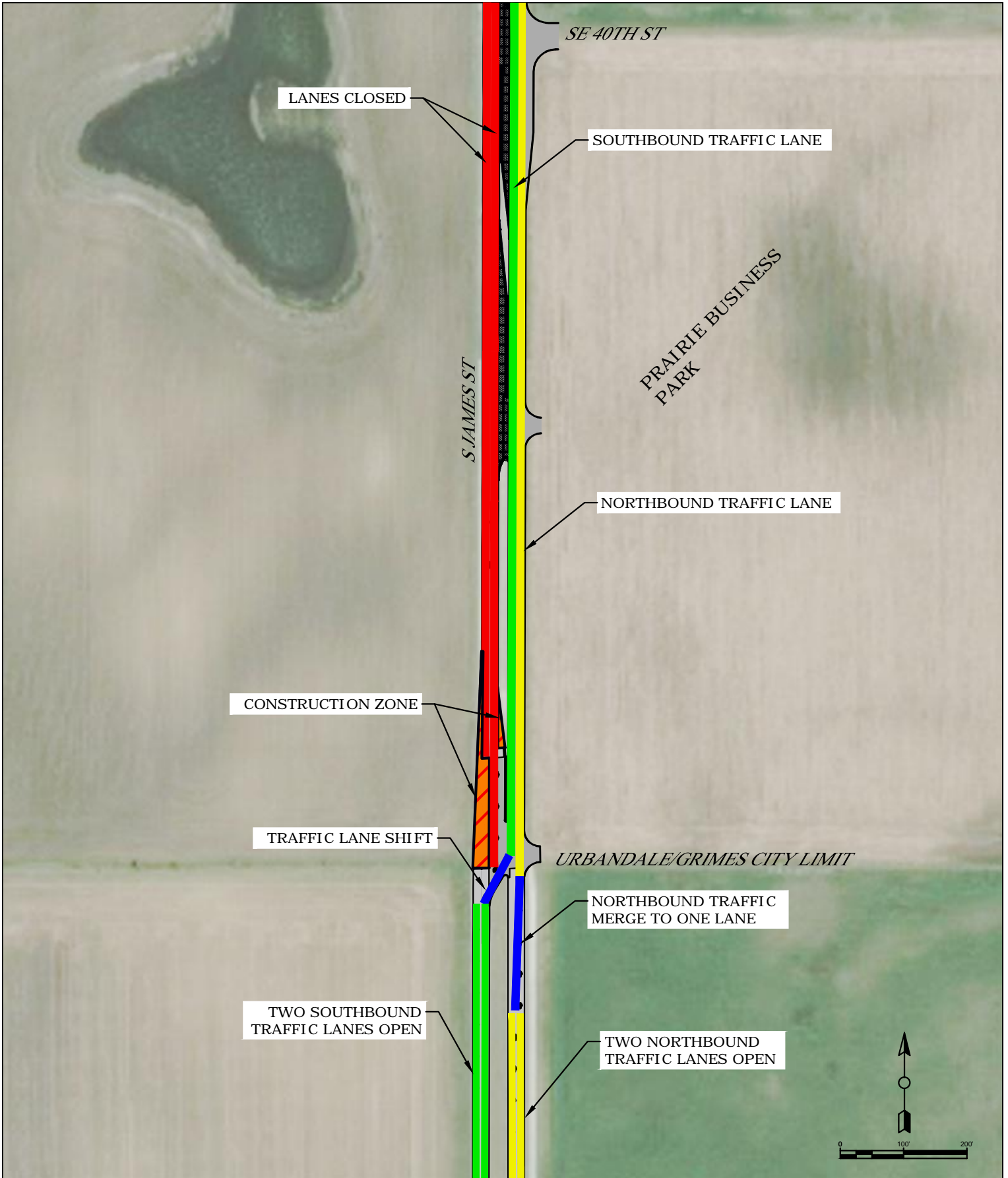
S JAMES & SE 37TH ST IMPROVEMENTS PROJECT PHASE 5A TRAFFIC CONTROL
